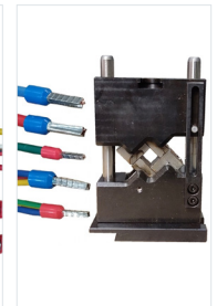
Insulated Ferrule Mold
